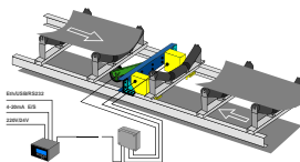
Integrating scale
