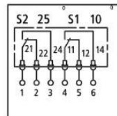
Connector strips
